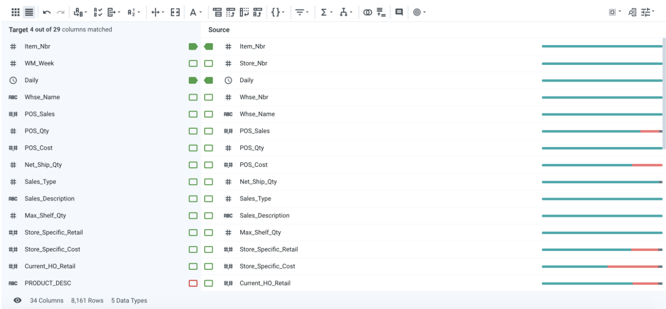
Figure: RapidTarget Panel in Column Browser
