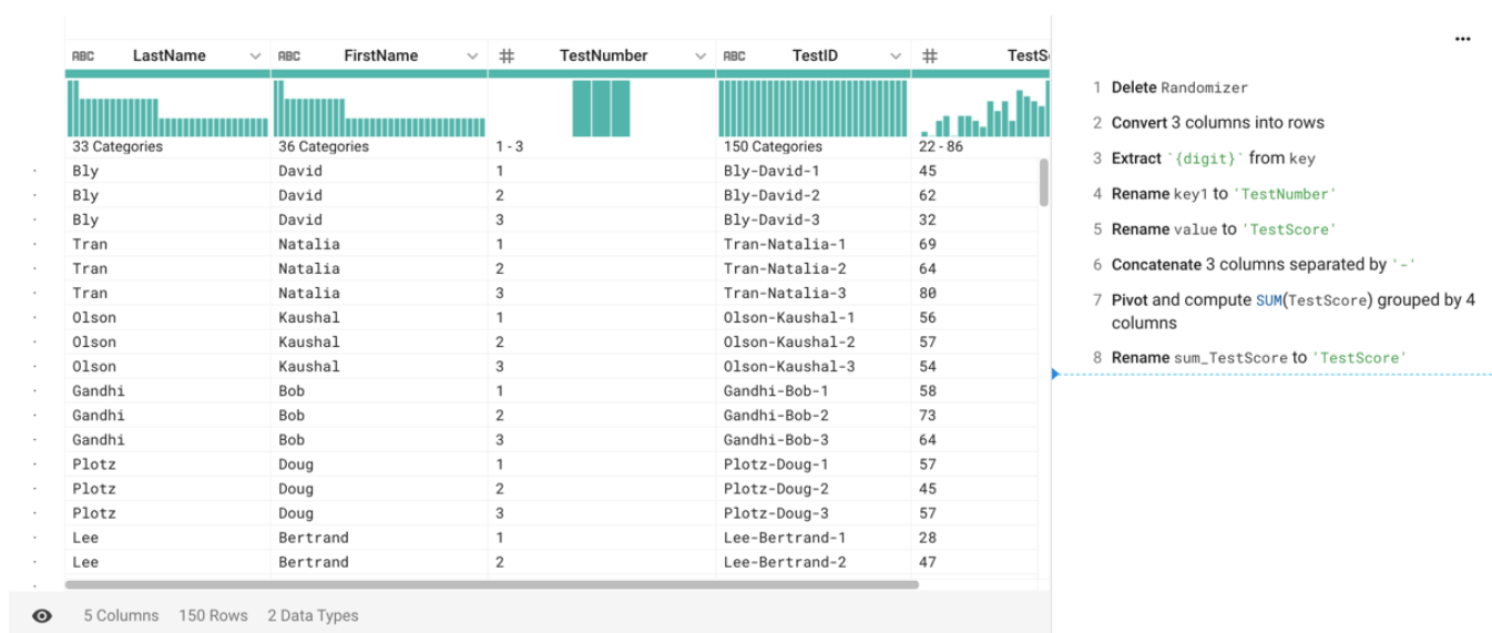
Figure: Single column of test scores
