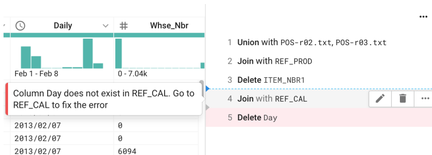
Figure: Dependency error in the Recipe panel
